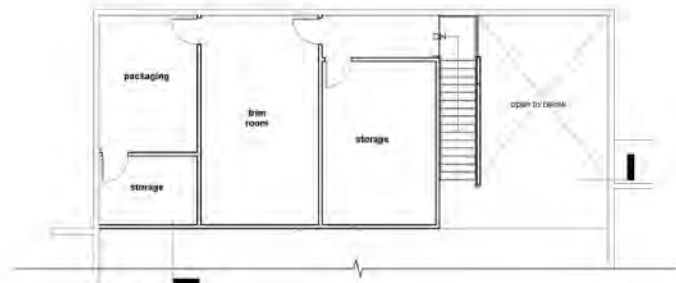
Second Floor
